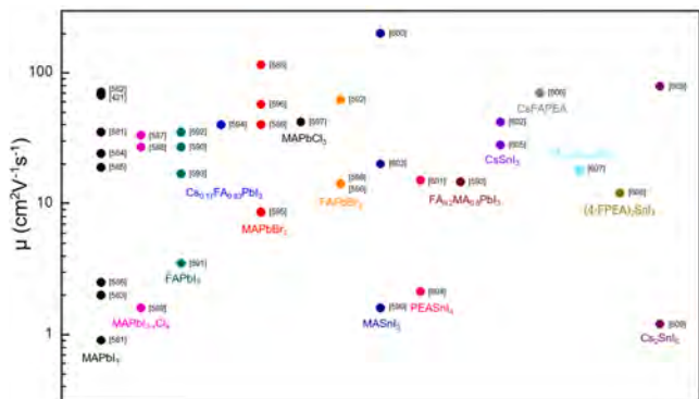
Fig. 37. Static sum of mobility values probed by experiments for different halide perovskite compositions.
