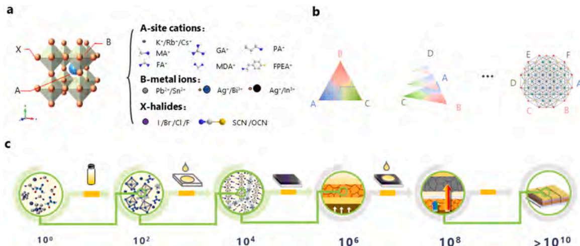
Fig. 31. Illustration of the complexities in metal-halide perovskites. (a) Crystal structure and typical ions of metal-halide perovskite materials. (b) Ternary phase diagrams represent the combinatorial complexity of alloying at the A, B, and X sites. (c) Schematic of the multidimensional aspects in fabricating perovskite solar cells, from precursor solutions, thin-film deposition, crystallization, and device fabrication. The possible combinations will be more than 10 10 .
