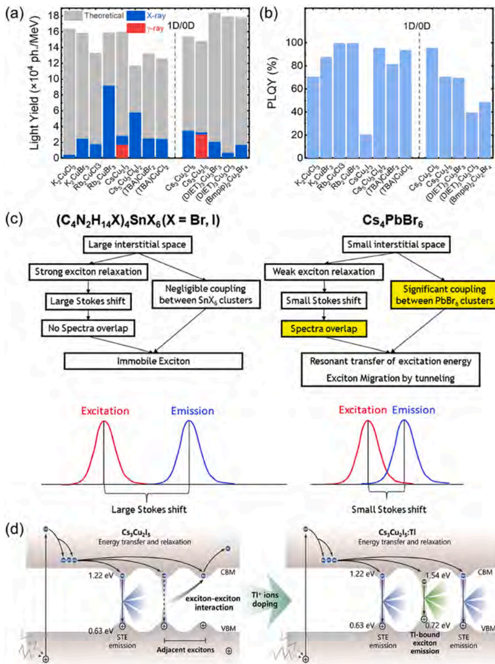
Fig. 27. (a) Light yields and (b) PLQYs of low-dimensional copper-based halide scintillators. (c) Illustration of the mechanisms that lead to the immobile excitons in (C_4N_2H_{14}X)_4SnX_6 ( X = Br, I ) and the mobile excitons in Cs_4PbBr_6 . (d) Theoretical single-particle electronic energy levels and scintillation emission mechanisms in Cs_3Cu_2I_5 and Cs_3Cu_2I_5:Tl under ionizing radiation [473,474].
