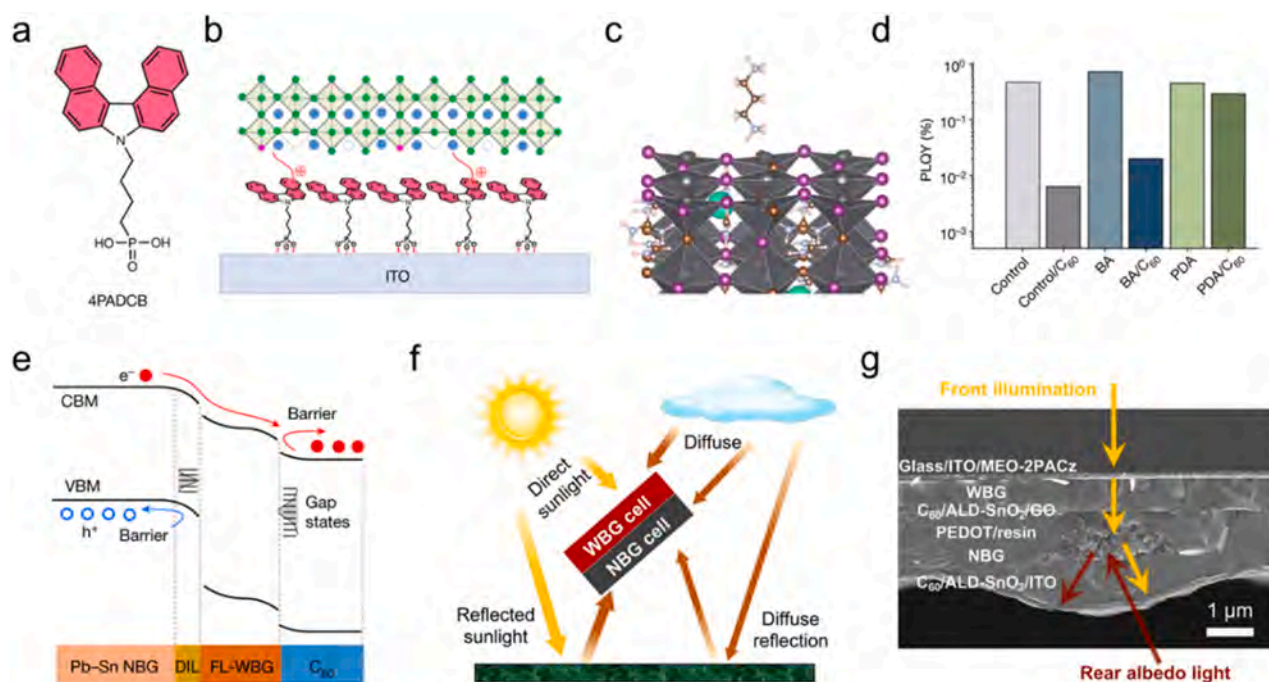
Fig. 14. (a) Molecular structure of 4PADCB [141]. (b) Schematic of the interconnection between ITO, 4PADCB and perovskite [141]. (c) Schematic crystal structure of perovskite surface treated with a PDA ligand [45]. (d) Photoluminescence quantum yield (PQY) data from control, BA- and PDA-treated films, with and without C 60 , on an ITO/hole selective layer substrate [45]. (e) Energy diagram for the Pb-Sn PSC with 3D/3D bilayer perovskite heterojunction. The heterojunction enables holes to be driven away (blue lines) and accelerates the drift of electrons (red lines) into the C 60 transport layer, thereby reducing the non-radiative recombination at the defective surface layer. The black and blue lines denote the non-radiative recombination pathways and the directions of carrier drift, respectively [163]. (f) Sketch of light absorption in a bifacial all-perovskite tandem device with additional albedo light [194]. (g) Scanning electron microscope (SEM) image of a bifacial all-perovskite tandem device [194].
