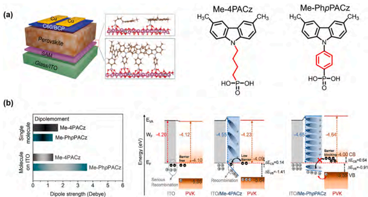
Fig. 8. a. Molecular structures of Me-4PACz and Me-PhpPACz and their stacking simulations in the device. b. Molecular dipole moment variation and energy alignment of Me-4PACz and Me-PhpPACz [97].
