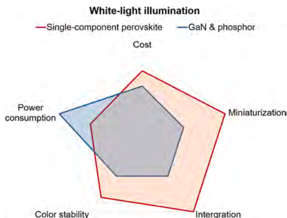
Fig. 19. A comparative analysis of the performance metrics between white light-emitting diodes (WLEDs) utilizing either single-component perovskite (SCP) or a hybrid design integrating GaN chips with a phosphor coating. The SCP-based WLEDs demonstrate noteworthy color stability, lower manufacturing costs, and a capacity for miniaturization and integration. However, it is worth mentioning that these advantages are counterbalanced by their power consumption, which lags significantly behind GaN-based WLEDs.
