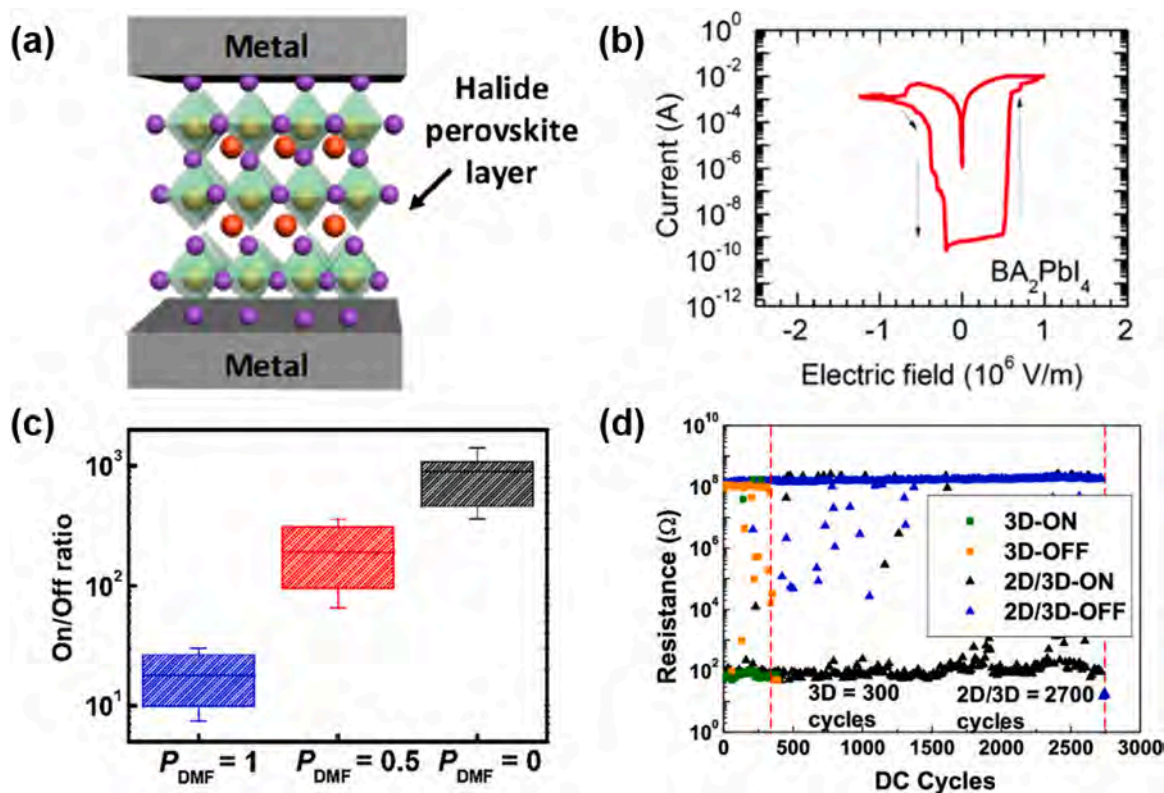
Fig. 41. (a) Schematic of the RSM structure with halide perovskites. Reproduced with permission from [ref. 656]. Copyright 2022, American Chemical Society. (b) I–V curve of the RSM utilizing the 2D BA 2 PbI 4 . Reproduced with permission from [ref. 661]. Copyright 2017, The Royal Society of Chemistry. (c) Variations in the on/off ratio across different V_{DMF}/V_{DMSO} . Reproduced with permission from [ref. 664]. Copyright 2022, American Chemical Society. (d) Endurance performance of the 2D/3D halide perovskite heterojunction. Reproduced with permission from [ref. 665]. Copyright 2020, American Chemical Society.
