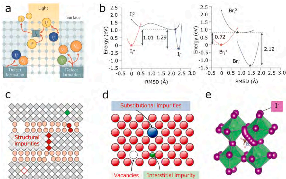
Fig. 2. a, Illustration of the migration path of I^- ions in MAPbI_3 crystal [30]. b, The relative energy diagram of the gap between bromine and iodine ions which indicates that the negative bromine ion gap is more difficult to oxidize than its iodine homologues [30]. c, Schematic diagram of phase purity and crystal orientation structure [24]. d, Schematic diagram of possible doping sites in 3D perovskite, especially doping sites within grain boundaries [34]. e, Schematic diagram of ion ( I^- ) migration channels in MAPbI_3 [36].
