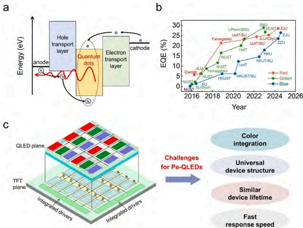
Fig. 21. a, Working principle of multi-layer Pe-QLEDs. b, Evolution curves of the peak EQEs in reported red [311,313–318], green [307,310,319–327], and blue [308,310,312,328–333]. Pe-QLEDs. c, Schematic illustration of the proposed structure of active matrix Pe-QLED displays and the challenges faced by Pe-QLEDs. Adapted with permission from Dai et al., Adv. Mater. 29, 1607022 (2017). Copyright 2017 John Wiley and Sons.
