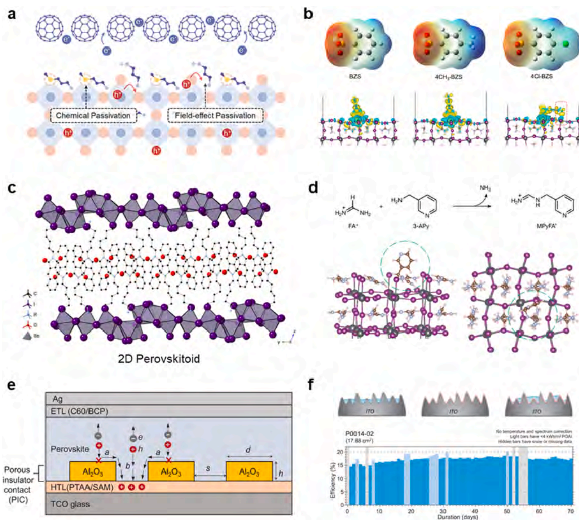
Fig. 4. a, Schematic of the perovskite surface without passivation and with both chemical and field-effect passivation [44]. b, Structure and electrostatic potential of BZS, 4CH 3 -BZS, and 4Cl-BZS ligands and atomic structures of ligand adsorbed in a preferred orientation on the perovskite surface [77]. c, Crystal structure of 2D perovskitoid (A 6 BfP) 8 Sn 7 I 22 . Carbon, nitrogen, oxygen, tin, and iodine are shown in black, blue, red, lavender, and purple, respectively. Hydrogens are omitted for visual clarity [78]. d, Condensation reaction scheme of FA + and 3-APy and DFT modelling of the atomic structures of the perovskite with charged V i and 3-APy modification. The brown, blue, pink, black and purple spheres denote C, N, H, Pb and I atoms, respectively [72]. e, Schematic description of the “porous insulator contact” device structure with Al 2 O 3 passivation at the perovskite/SAMs interface [73]. f, Illustrations for the different HTMs on the ITO substrate and the outdoor stability of the minimodules based on the hybrid hole transport materials [75].
