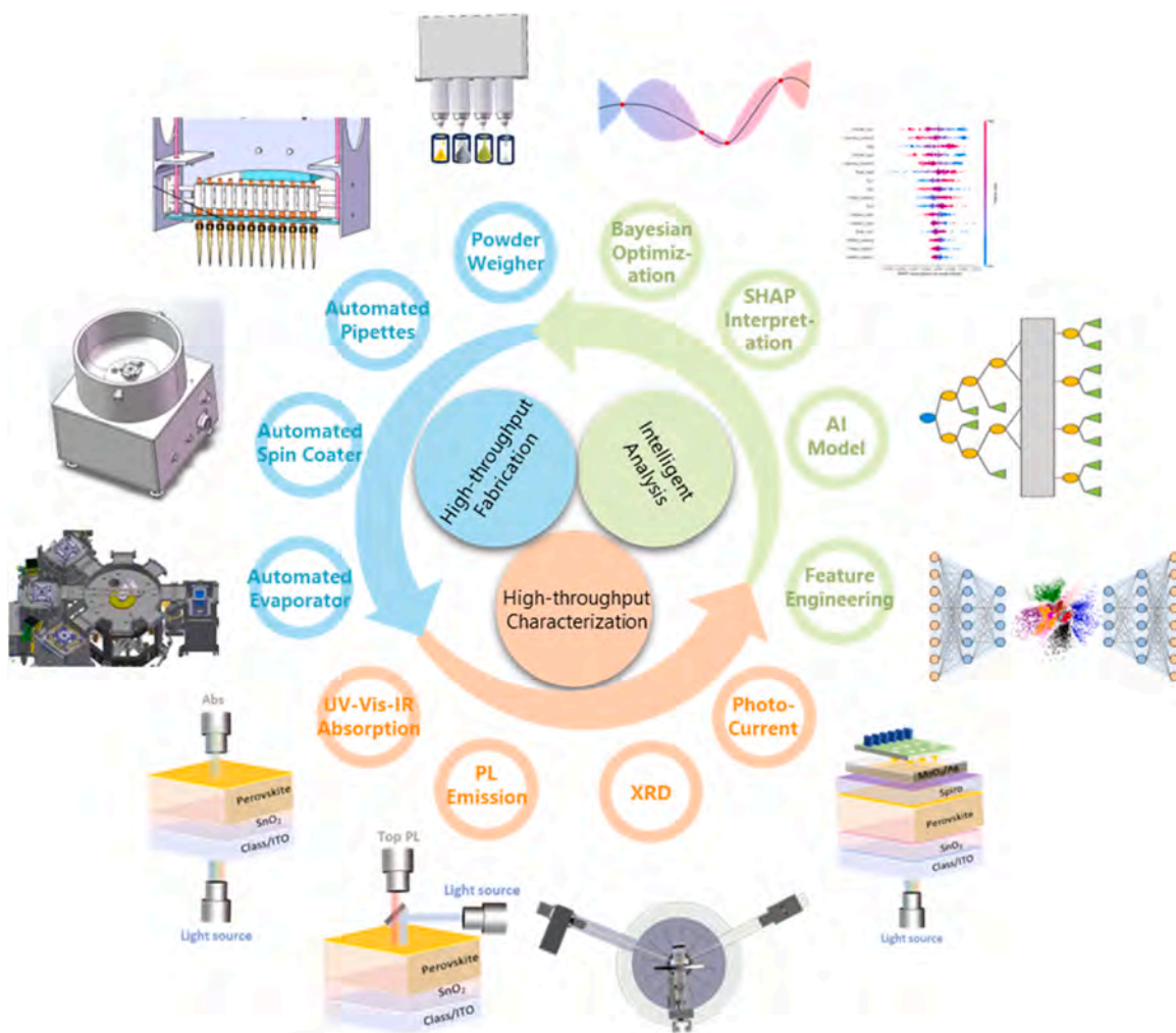
Fig. 32. Schematic of a high-throughput intelligent experimental platform for solution-processed semiconductor research. The system integrates automated fabrication (pipettes, weighers, spin coaters, evaporators), comprehensive characterization (UV-Vis, PL, XRD, photo-current), and intelligent analysis (AI models, Bayesian optimization [540], feature engineering). This closed-loop setup enables efficient data-driven optimization for rapid material discovery.
